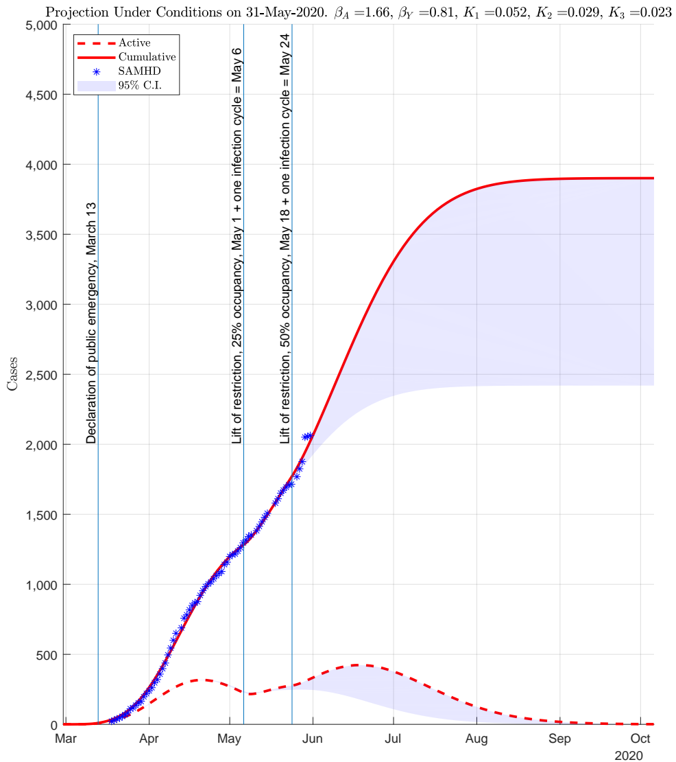
Figure 0.0-1: IMPORTANT: 776 congregated cases were removed from analysis on 31-May-2020. These cases are not included in projections. File: SanAntonio31-May-2020-EVOLUTION
